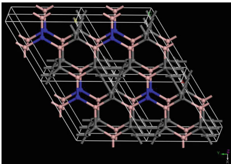
Fig. 1 View of the Wellsean trigohexagonite lattice in space group P-6m2 (#187), from a perspective along the c -axis: 3-connected vertices are blue and pink, 4-connected vertices are gray
