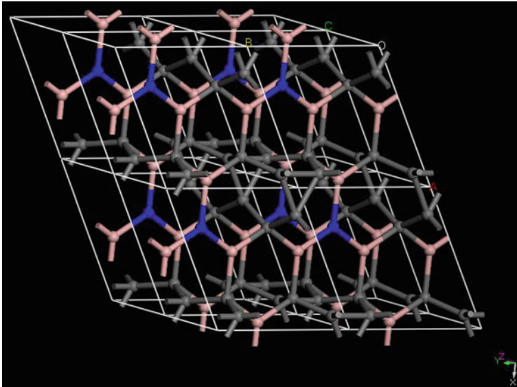
Fig. 2 View of Wellsean trigohexagonite lattice in space group P-6m2 (#187), from the perspective of the ab -plane: 3-connected vertices are blue and pink, 4-connected vertices are gray
